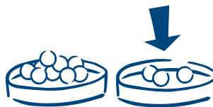
few (9.7)
